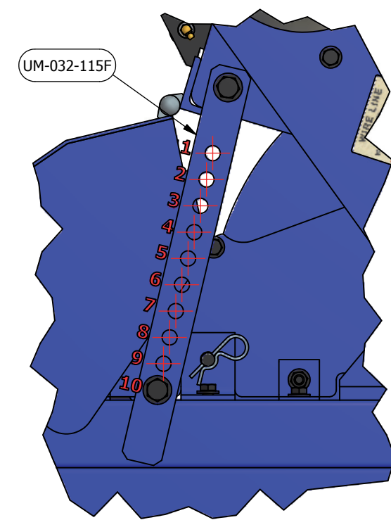
DETAIL B
