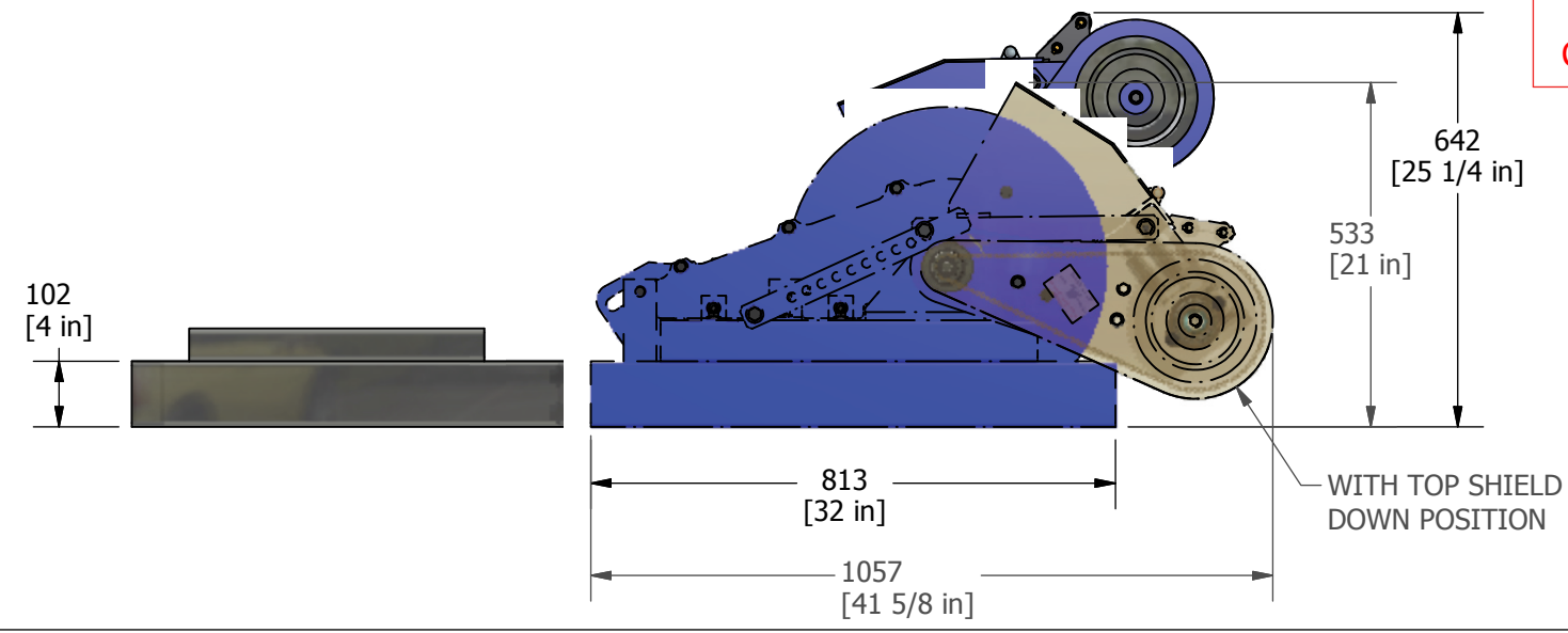
HOIST WIRE LINE OVERALL DIMENSION (10 000' / 3048 Metre)
